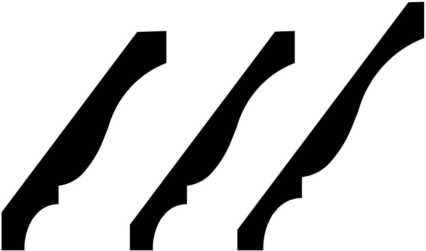
CROWN WM 47 11/16 x 4-5/8 FJ PINE – R/L 109640
