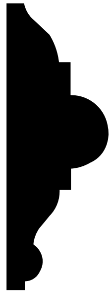
CHAIR RAIL WM 300 1-1/16 x 3 FJ PINE - R/L 104227
