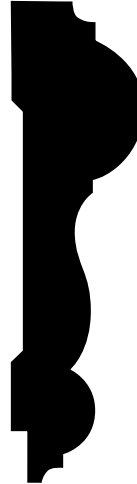
CHAIR RAIL LWM 298 11/16 x 2-1/2 3/8" RABBETED PINE - R/L 280946
