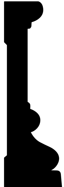
CASING LGM 7 1-1/16 x 3-1/2 FJ PINE - R/L 266877 FJ PINE - 6/8 228707 PINE - R/L 266881 PRMD - R/L 506176 PRMD - 6/8 608297
